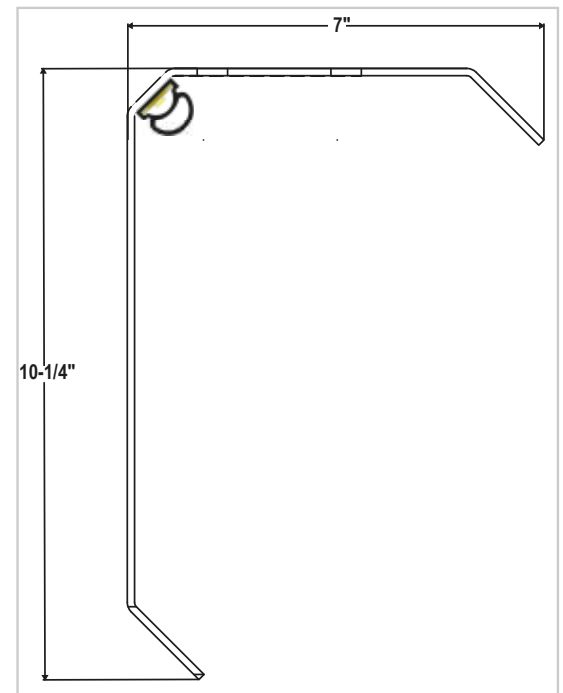
FIXTURE PROFILE
